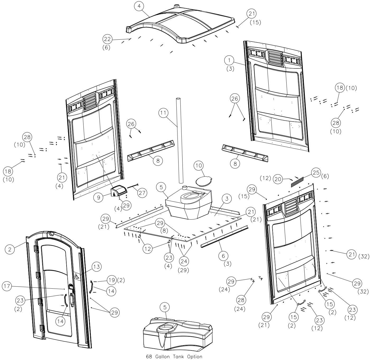
68 Gallon Tank Option
